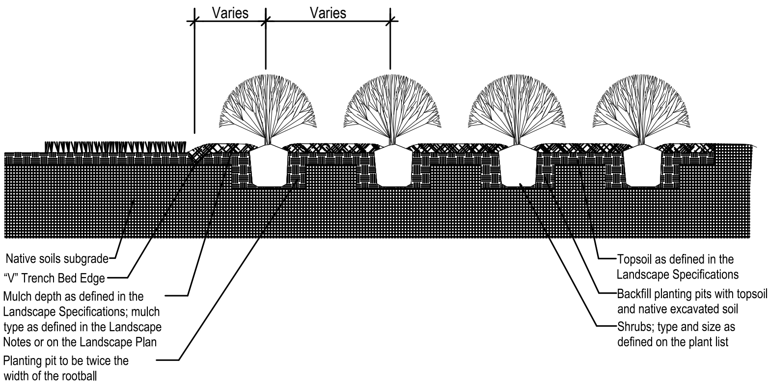
SHRUB BED PLANTING DETAIL SCALE: NTS
