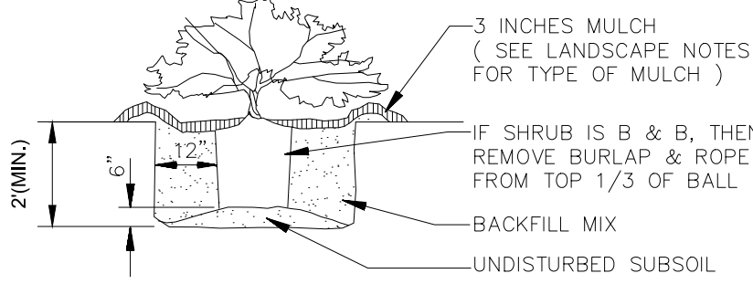
SHRUB PLANTING N.T.S.
