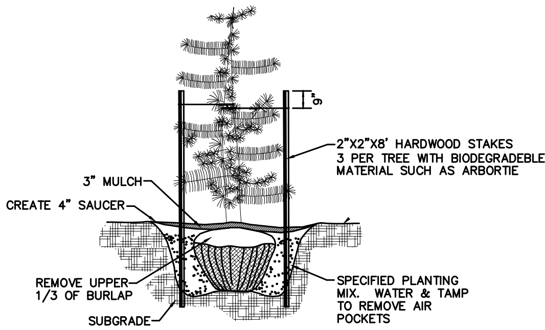
EVERGREEN TREE PLANTING DETAIL SCALE: NTS
