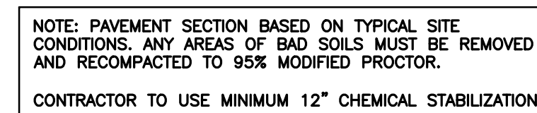
STANDARD DUTY ASPHALT TYPICAL PAVEMENT SECTION
