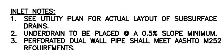
PIPE UNDERDRAIN AT STRUCTURES (TYPICAL INSTALLATIONS) NO SCALE
