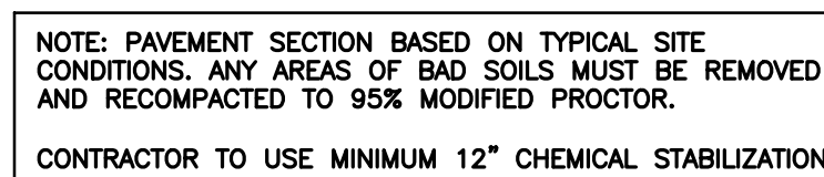
HEAVY DUTY ASPHALT TYPICAL PAVEMENT SECTION NO SCALE
